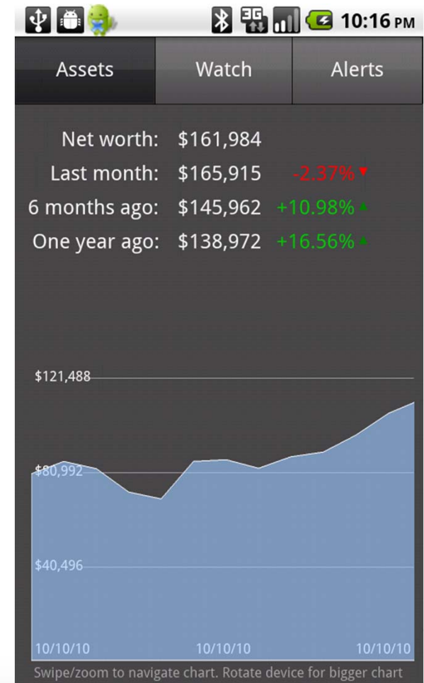
s:TabbedApplication
