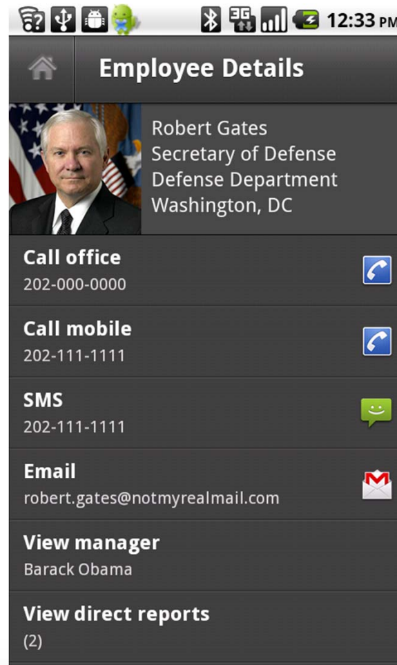
s:ViewNavigatorApplication
