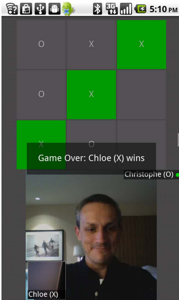
s:Application
